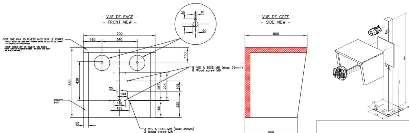
Fig. 1: Dimensional drawing CBA 240 S
