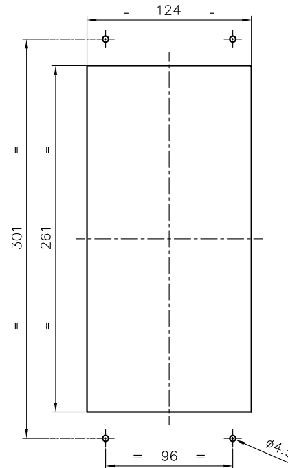
- ENCASTREMENT - - DIMENSIONS WALL MOUNTING -
