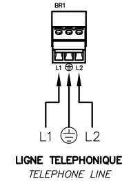
- RACCORDEMENT - - CONNECTION -
